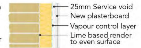
Internally insulated Stone Wall
