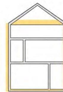
Hybrid Approach
