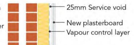
Internally insulated brick cavity
