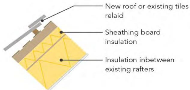
Rafter insulation detail
