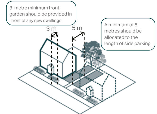
Figure 38: Illustrative diagram showing the indicative layout of and minimum dimensions of on-plot side parking, parking bays should be set slightly behind main building frontage to minimise visual impact on streetscapes.
