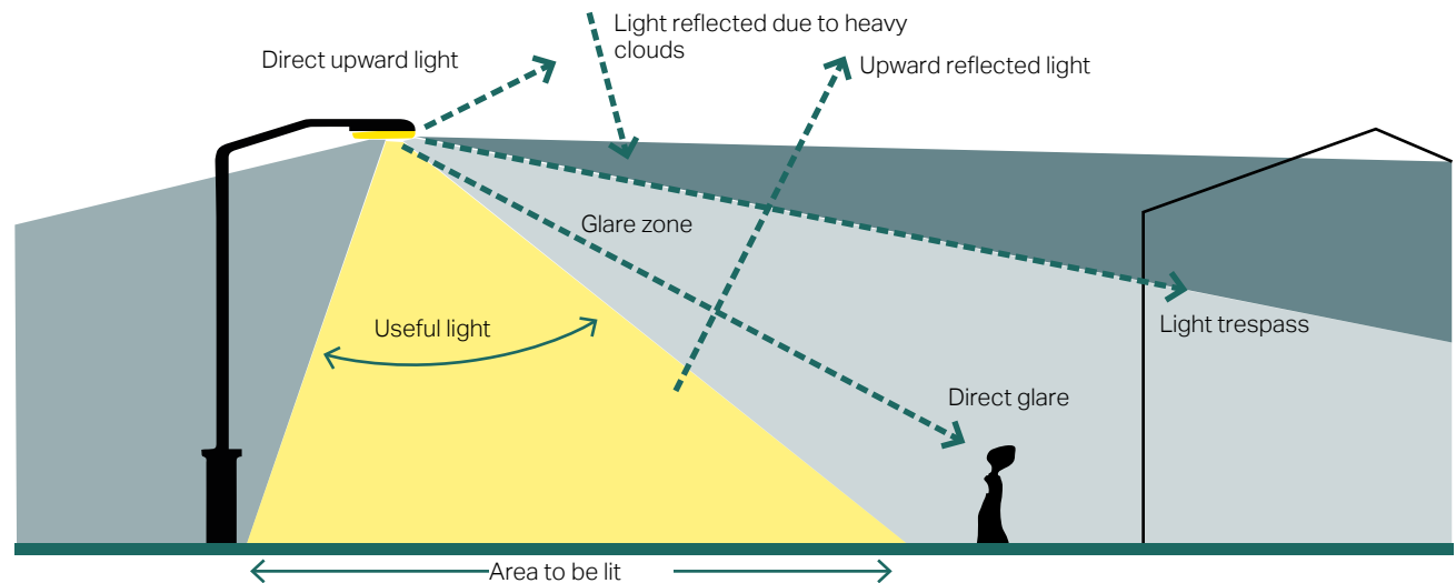
Figure 54: Diagram to illustrate the different components of light pollution and what 'good' lighting means for dark skies.
