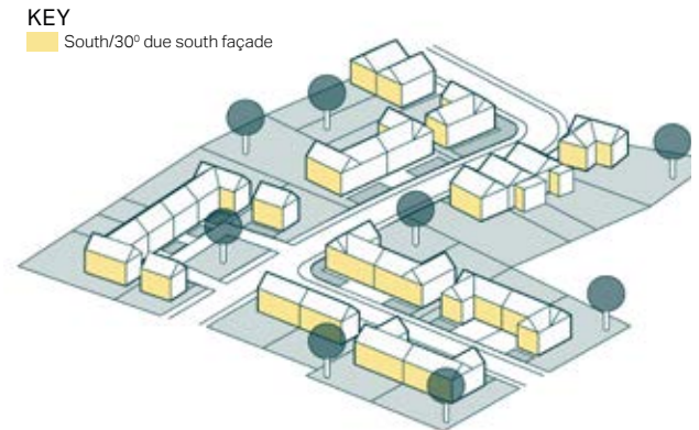
Figure 64: Elevations that would benefit from passive solar gain
