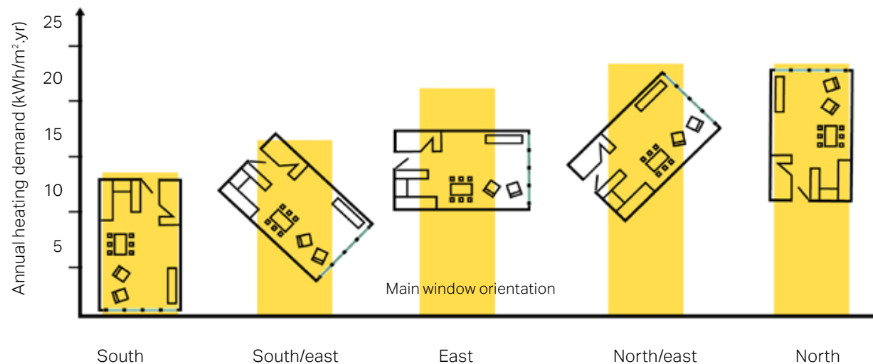
Figure 65: An illustrative graph showing solar orientation of a room against the annual heating demand.
