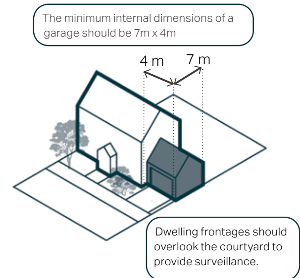
Figure 41: Illustrative diagrams showing the indicative layout of garage parking.
