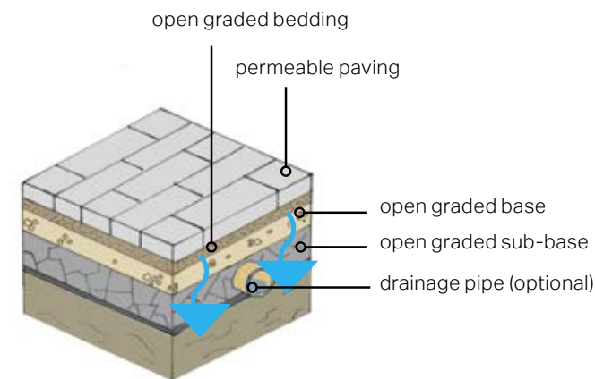
Figure 56: Diagram illustrating the function of a soak away.
