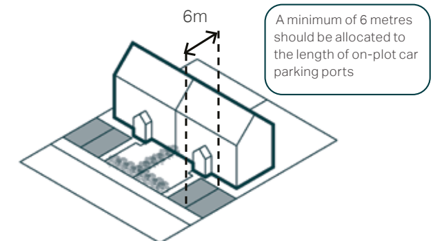
Figure 39: Illustrative diagram showing an indicative layout and minimum dimensions of on-plot front parking,
