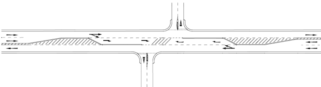
Figure 2.5N1d Staggered junction layouts at changeovers - non-conflicting layout
