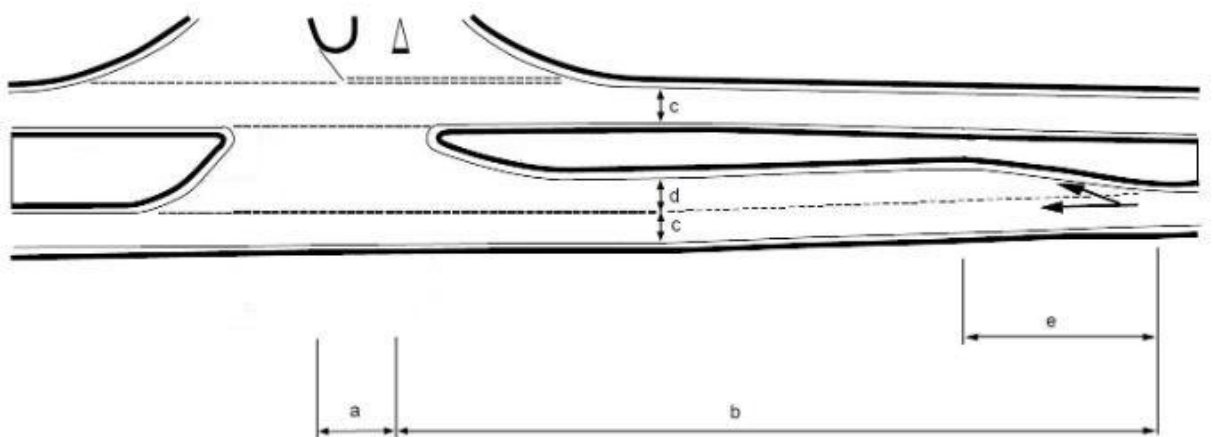
Figure 6.3d Major / minor priority junctions with SLD
